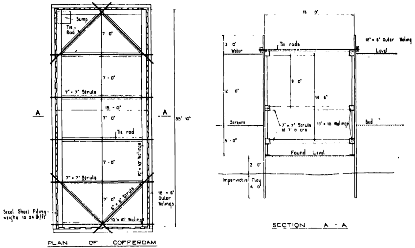
Fig. 151.—Typical Sheet-Pile Cofferdam.
